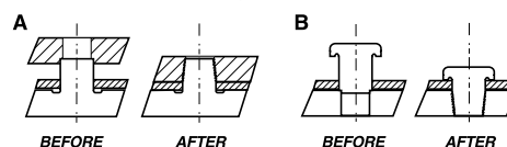
Figure 3. Variations of Basic Joint
