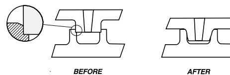
Figure 2. Stud in Boss or Blind Hole
