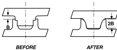
Figure 6. Double-Stepped Stud Weld
