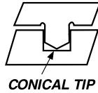
Figure 5. Stud Weld with Energy Director
