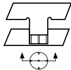
Figure 4. Stud Weld with Vertical Energy Directors
