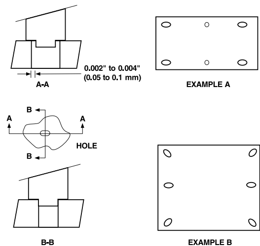
Figure 9. Variations for Large Parts
