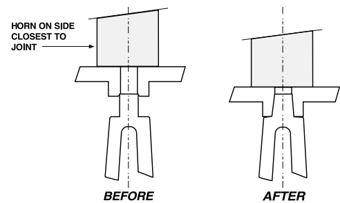
Figure 8. Optimum Horn Location
