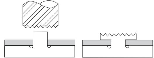
Figure 5. Knurled stake
