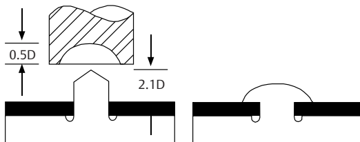
Figure 4. Dome stake
