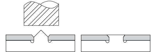
Figure 6. Flush stake
