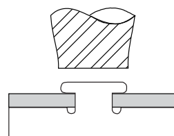
Figure 8. High-pressure stake
