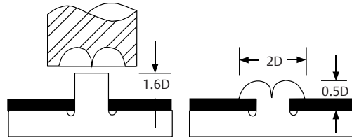
Figure 2. Standard profile stake
