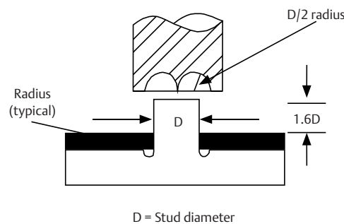
Figure 1. Relationship between stud and horn cavity
