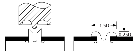
Figure 7. Hollow stake
