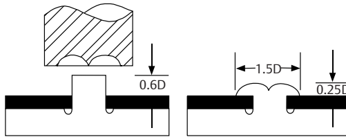
Figure 3. Low profile stake
