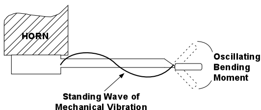
Figure 1 Standing wave of mechanical vibration during degating
