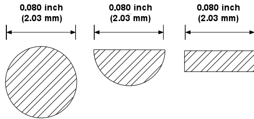
Figure 4 Gate size
