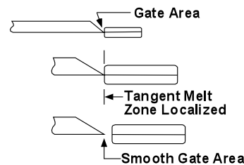
Figure 2 Correct gate design
