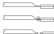
Figure 3 Incorrect gate design
