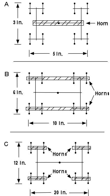
Figure 6 Horn size and placement
