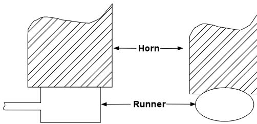
Figure 5 Maximizing horn-to-part surface area for best results
