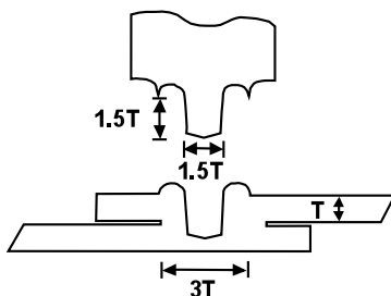
Figure 1. Standard Spot Welding Tip Design
